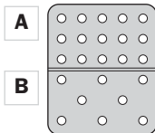
Pattern 114 Hole Diameter 0.3938"
